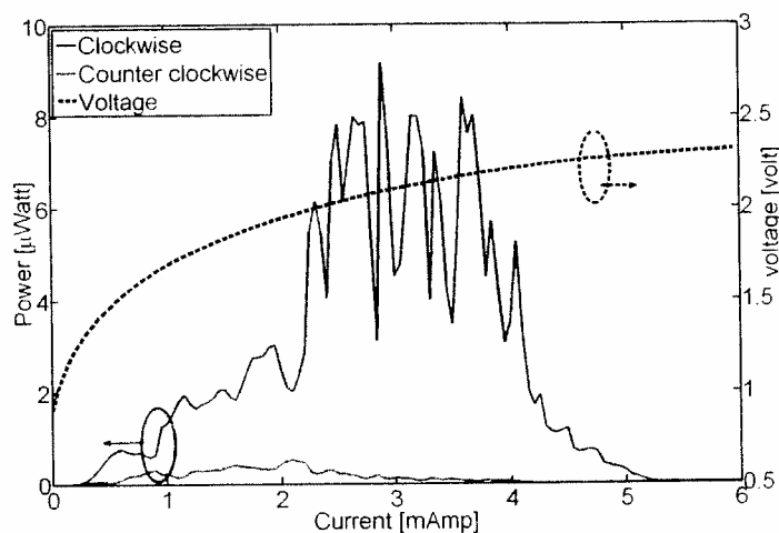
Figure 1: L-I & V-I curves of microdisc laser
