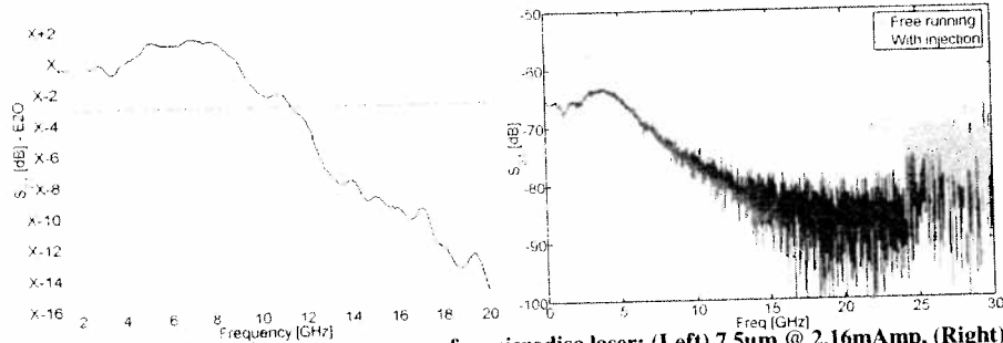
Figure 2: Small signal frequency response for microdisc laser; (Left) 7.5 \mu m @ 2.16mAmp, (Right) 10 \mu m @ 0.8mAmp
