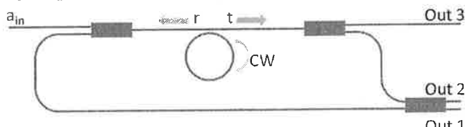
Figure 2: layout of the integrated interferometric circuit
