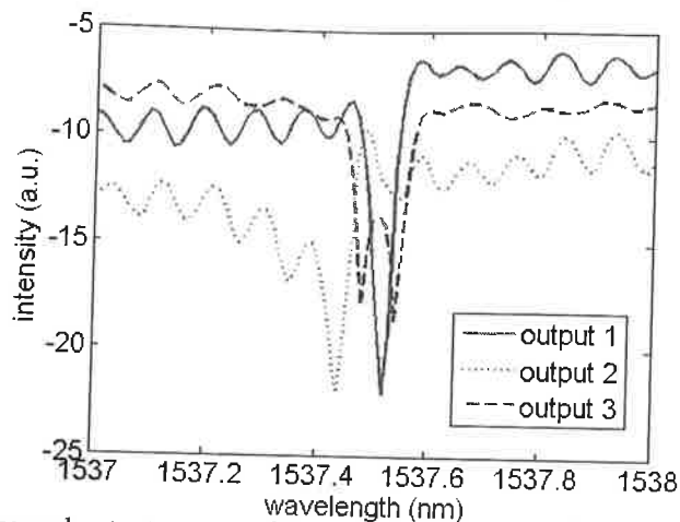
Figure 3: Measured output spectra of the circuit. Output one clearly shows the improvement of the resonance shape compared to the all-pass signal in output three.
